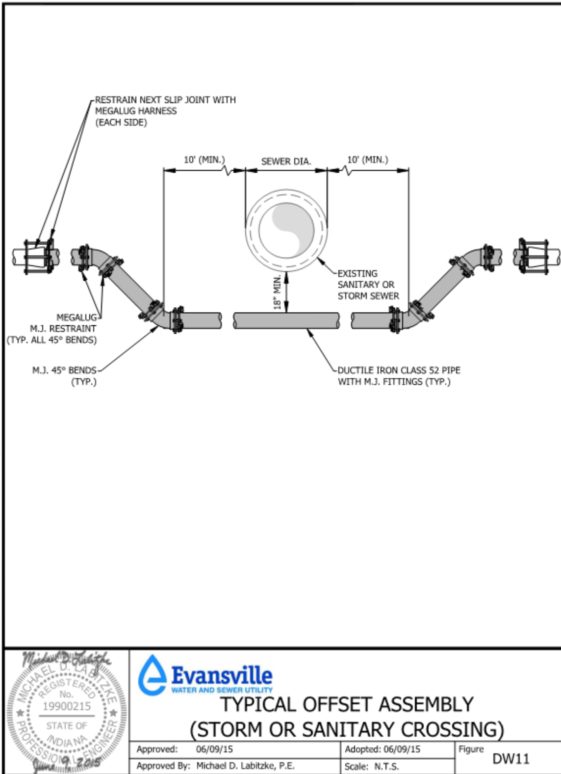
Figure 6-36: Detail DW-11 Typical Offset Assembly (Storm or Sanitary Crossing)
